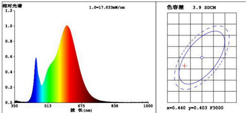
Attachment No. 1: Photometric test record of one lamp at initial measurement
